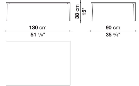
LXT130M
