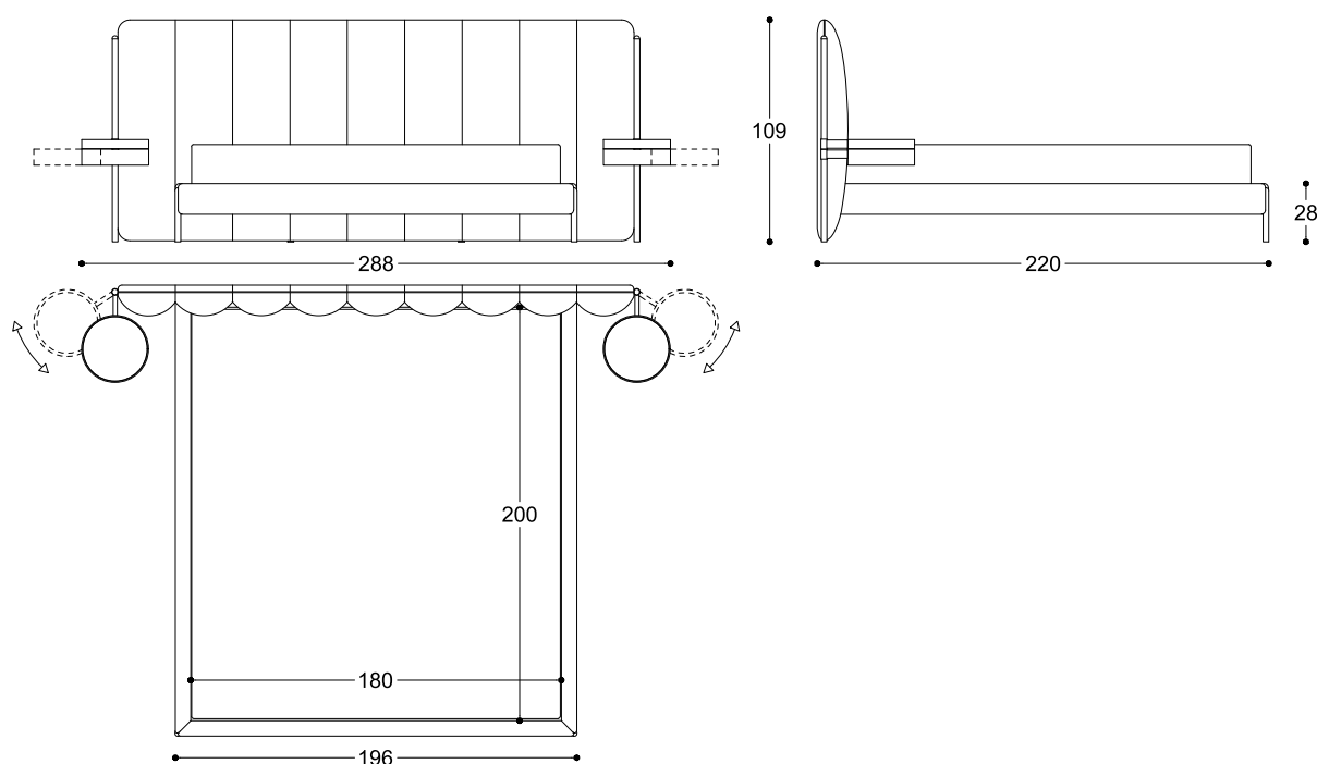
Article: Bed for mattress size 180 x 200 Code: IB180
