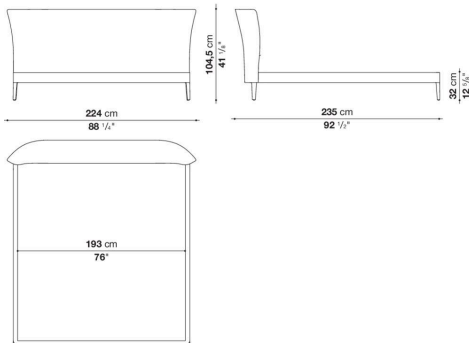
LFB193V
