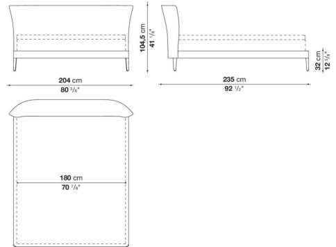
LFB180V
